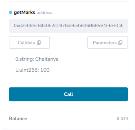
Fig 4: Retrieving stored student data using the getMarks() function
