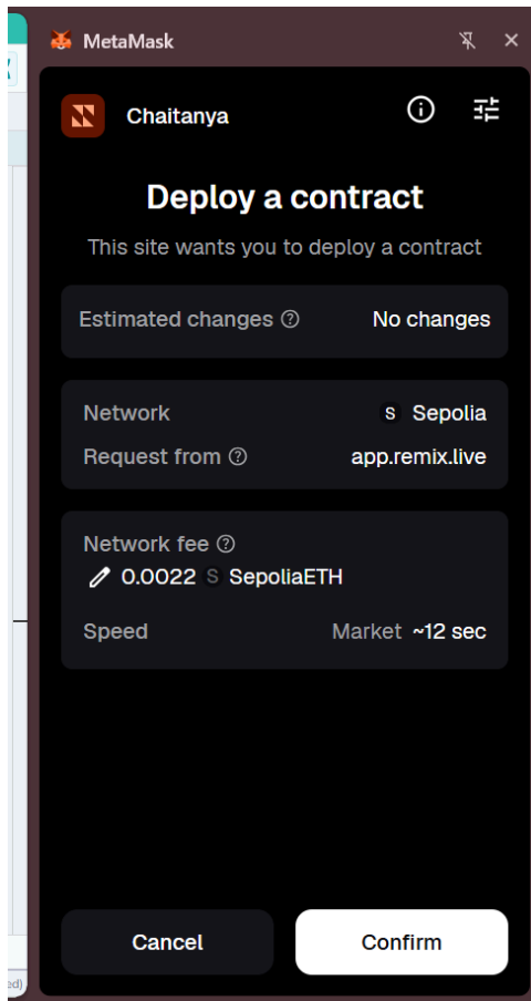
Fig 2: Confirming smart contract deployment transaction via MetaMask
