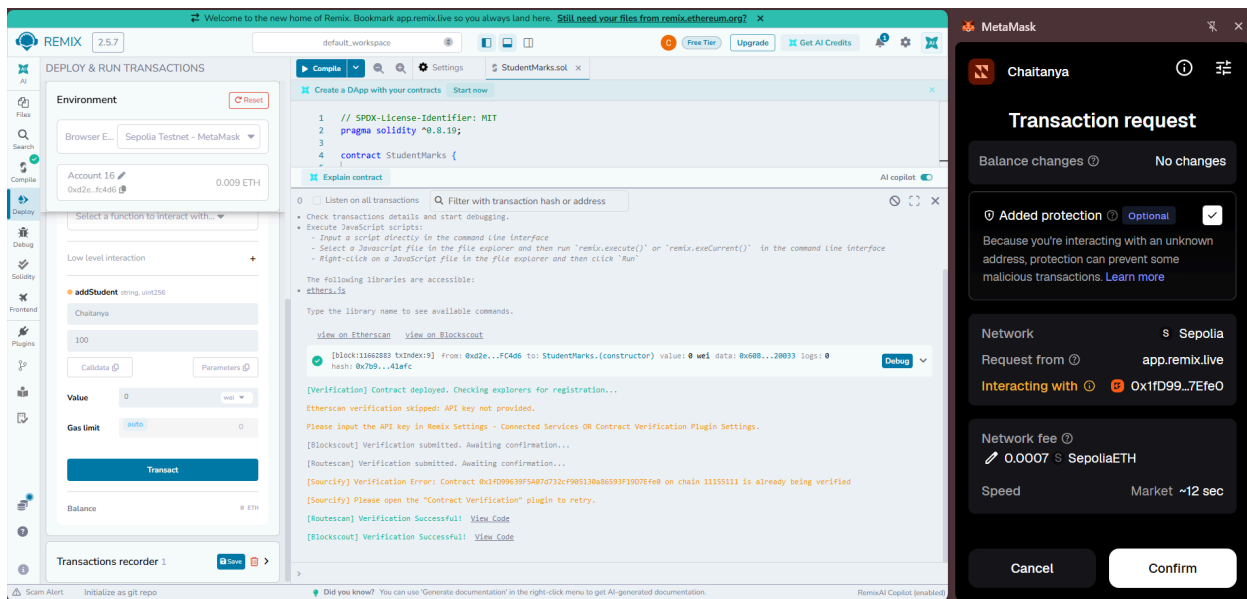
Fig 3: Calling the addStudent() function and confirming transaction on Sepolia
